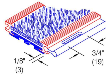
Perforated hinge
