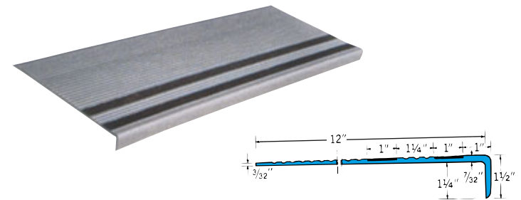
No. GS365 GRIT-STRIP KOROSEAL VINYL
